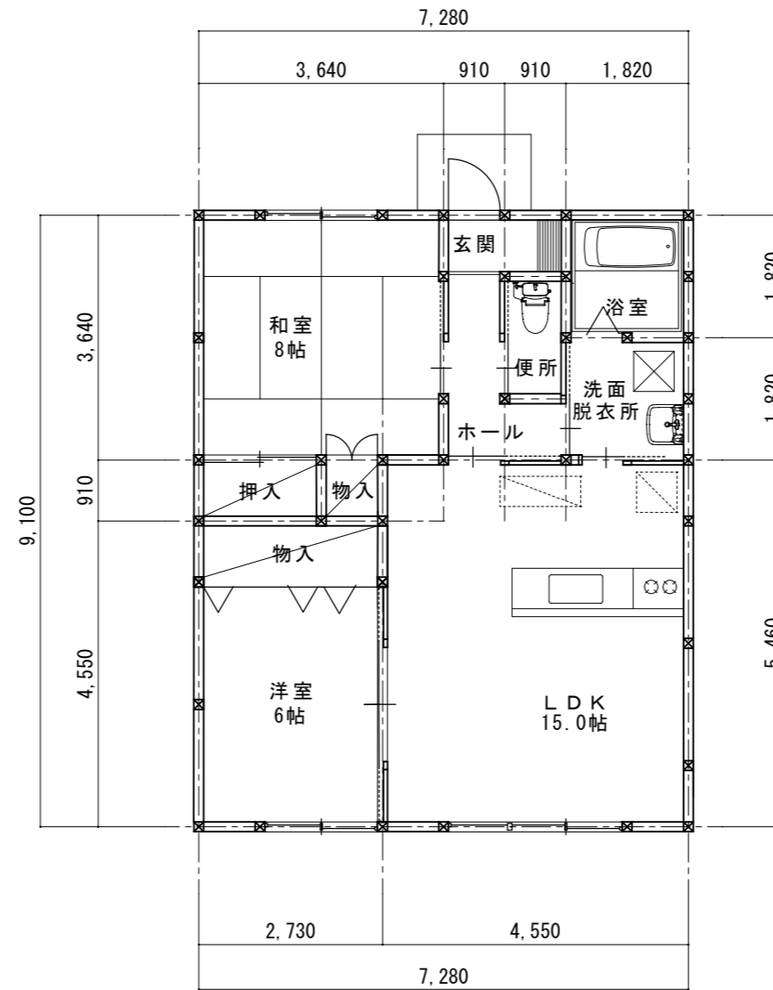
2LDK 66.2㎡
